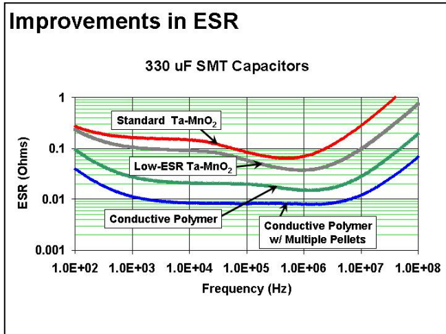
Figure 2. ESR versus frequency plots.
