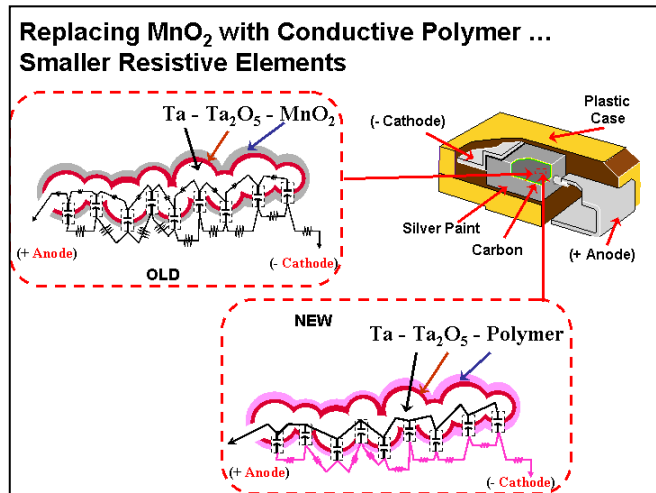
Figure 1. Cathode system change to conductive polymer.
