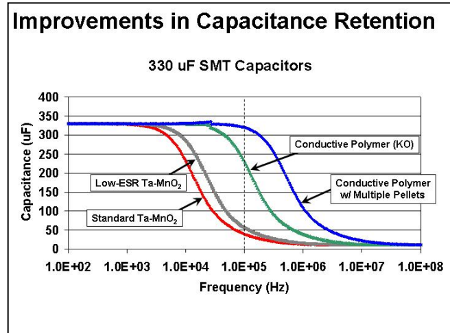
Figure 3. Capacitance versus frequency.
