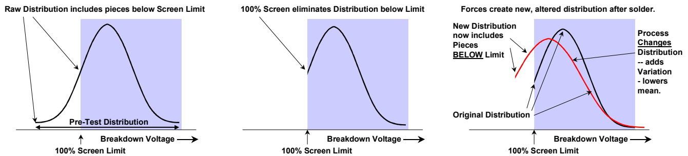
Figure 4. Raw distribution – Truncated Distribution by Screening – Shifted Distribution by solder process
