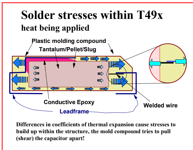
Figure 2. Mismatched coefficients of thermal expansion.
