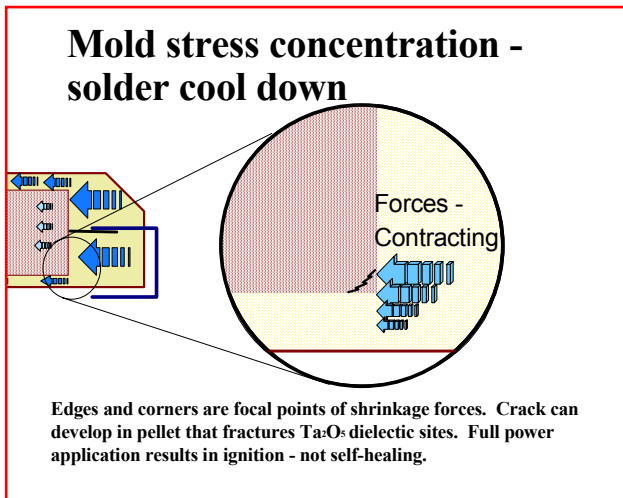
Figure 3. Contraction during cool-down after solder reflow.
