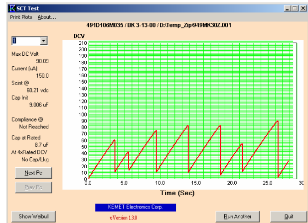
Figure 1. Multiple scintillations in tantalum capacitor. [1]
