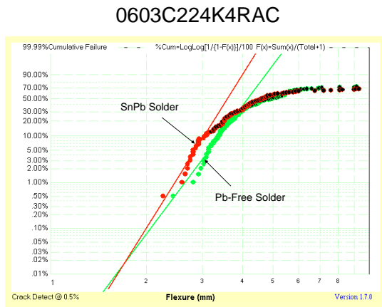
Figure 6. Flex performance 0603, .22 uF X7R, Pb-Free vs. SnPb Solders
