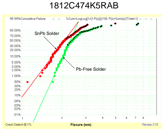
Figure 5. Flex performance 1812, .47 uF X7R, Pb-Free vs. SnPb Solders
