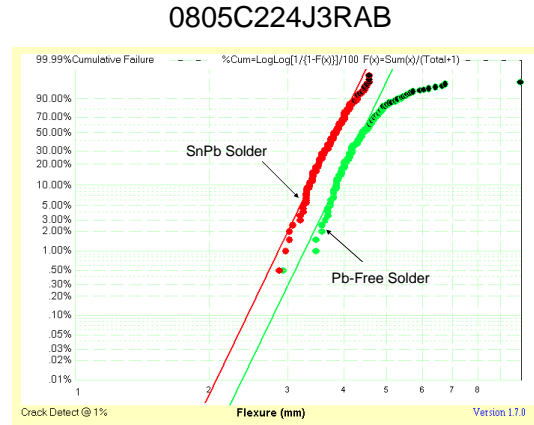
Figure 7. Flex performance 0805, .22 uF X7R, Pb-Free vs. SnPb Solders
