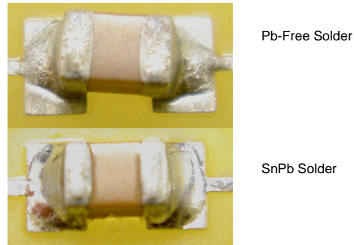
Figure 12. Solder Fillets
