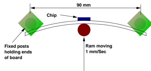
Figure 1. Flex Testing Fixture [1]
