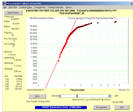
Figure 2. Weibull plot of 1812, .47 uF, X7R
