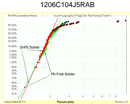
Figure 9. Flex performance 1206, .1 uF X7R, Pb-Free vs. SnPb Solders
