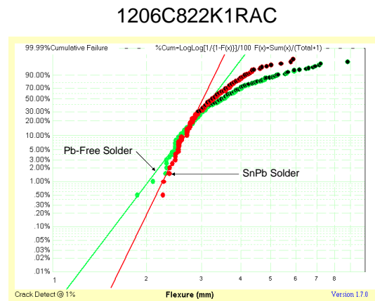
Figure 8. Flex performance 1206, 8.2 nF X7R, Pb-Free vs. SnPb Solders
