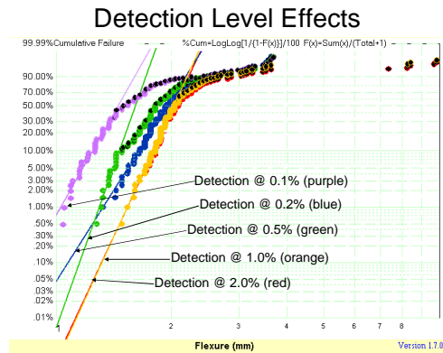
Figure 3. Different detection levels for the same part number
