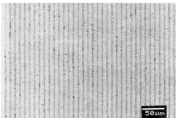
Figure 1a. SEM micrograph of polished surface of BME Y5V capacitor.
