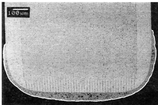
Figure 1b. Cross section of copper terminated and nickel plated BME X7R capacitor.
