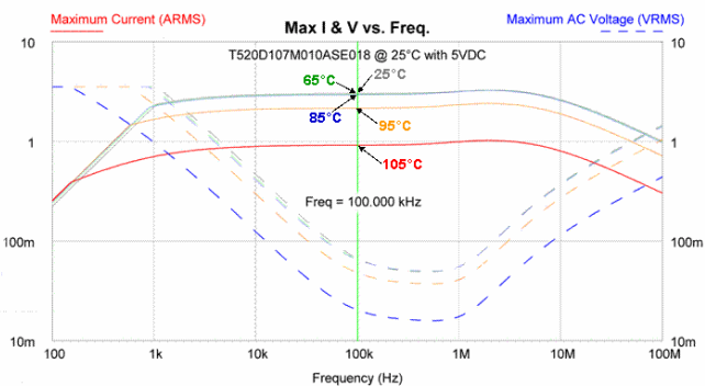
Figure 2. Ta-Polymer - Ripple current ( \Delta T_{max}=20^\circ C ) vs. ambient.
