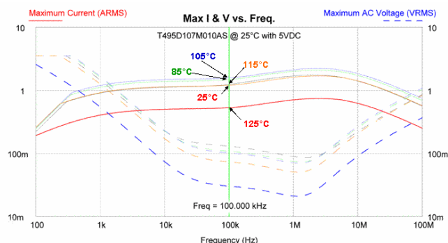
Figure 1. Ta-MnO 2 - Ripple current ( \Delta T_{max}=20^\circ C ) vs. ambient.
