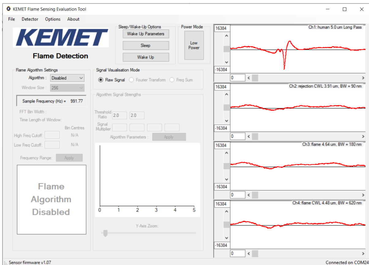
Figure 9 – Signal Viewers
